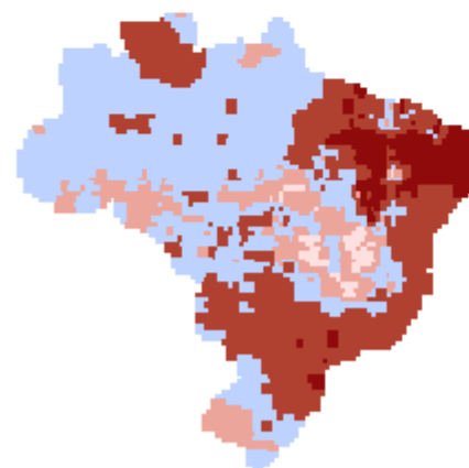
Crítico (BCCSM11-RCP8.5)
