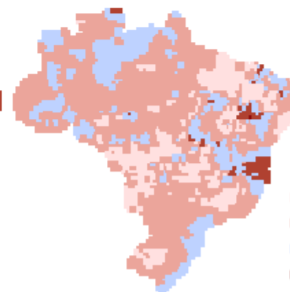
Otimista (CNRMCM5-RCP4.5)
